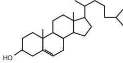
Cholesterol
