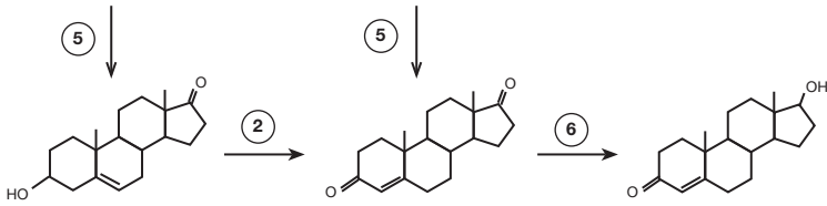
Dehydroepiandrosterone
