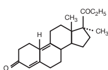
Promegestone (R5020)
